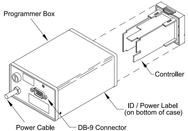
Figure 3 Exploded View
