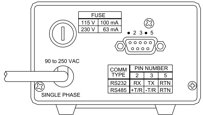
Figure 2 Rear View
