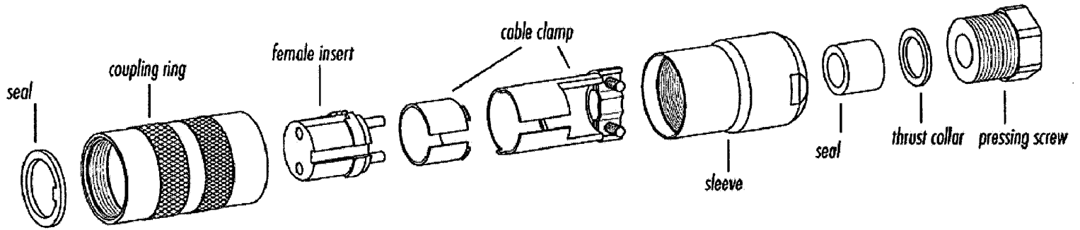
FEMALE CABLE CONNECTOR WITH CABLE CLAMP, CABLE OUTLET 4–6 mm
